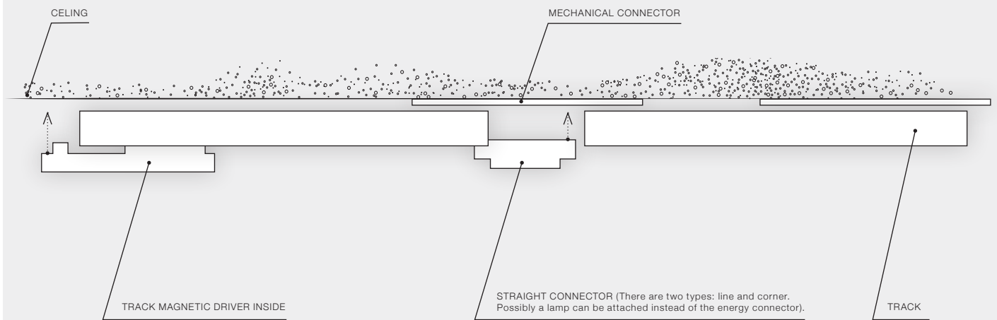
01 Insert the MECHANICAL CONNECTOR (B) into the TRACK (A).
