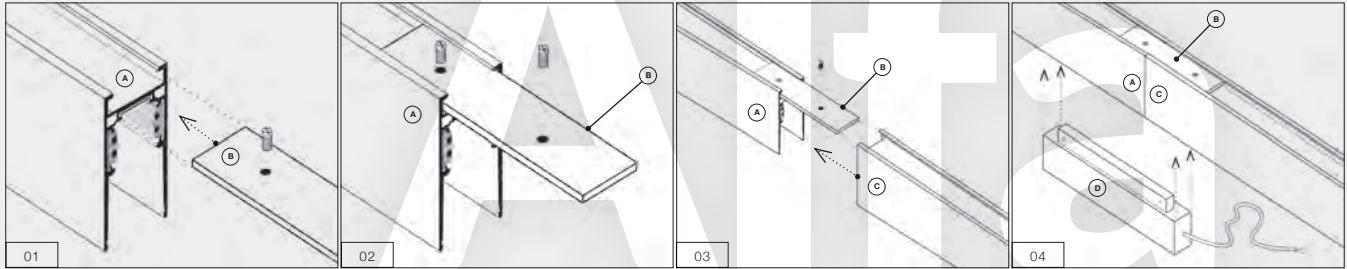
01 Insert the MECHANICAL CONNECTOR (B) into the TRACK (A).
